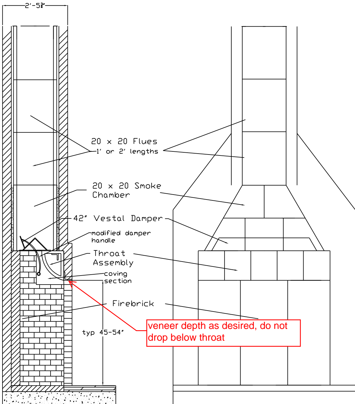
Elevation section
