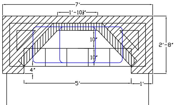
plan section
