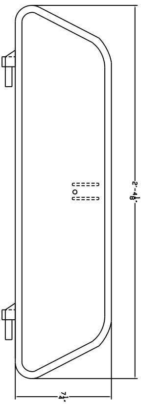
LARGE FLAT DAMPER VALVE PLATE
