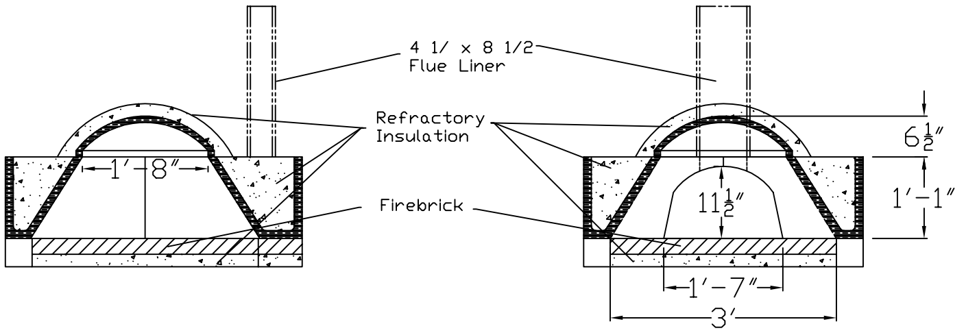
Section-Elevation
