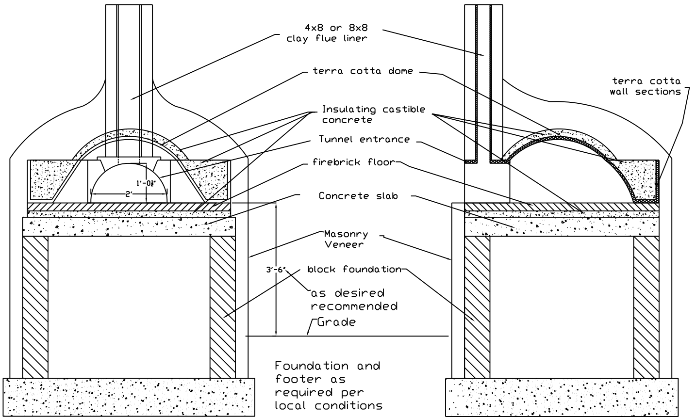
SECTION/ ELEVATION
