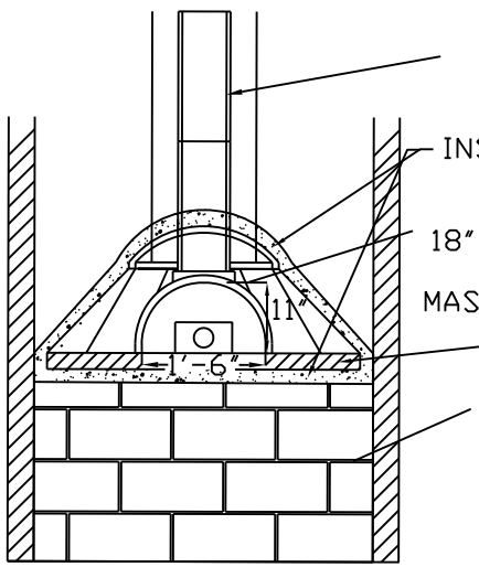
SECTION/ELEVATION
