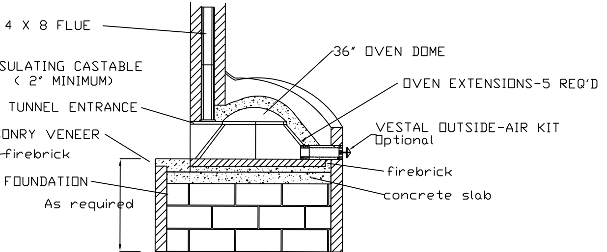
SECTION/ELEVATION
