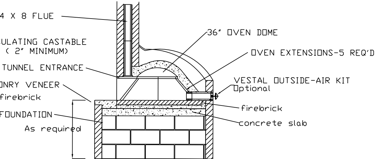
SECTION/ELEVATION
