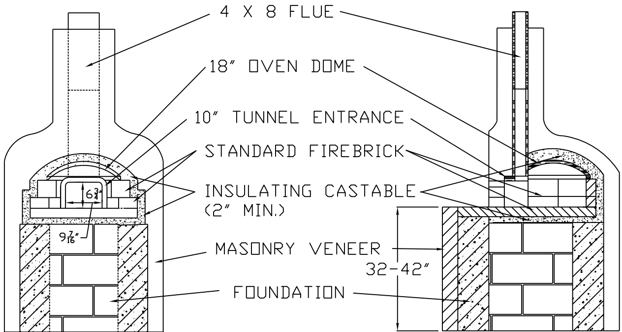
SECTION/ELEVATION
